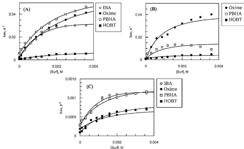
Figure 4. Simulated rate-surfactant profiles for the reaction of PNPA (A), PNPDP (B), and parathion (C) with different \alpha -nucleophiles [I] in the presence of cetyltriphenylphosphonium bromide micelles (lines are predicted values with model)
