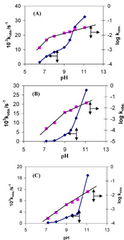
Figure 1. Plots of observed rate constant versus pH and log of observed rate constant versus pH for the hydrolysis of p -nitrophenyl diphenyl phosphinate by IBA (A), oxime (B), and PBHA (C) at 27 °C. This figure is available in colour online at www.interscience.wiley.com/journal/poc
