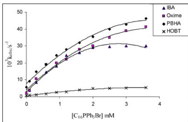
Figure 2. Rate surfactant plots of k_{\text{obs}} (rate constant) versus [surfactant] for the nucleophilic reaction of PNPA with different \alpha -nucleophiles [I]. This figure is available in colour online at www.interscience.wiley.com/journal/poc
