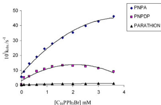
Figure 3. Rate surfactant plots of k_{\text{obs}} (rate constant) versus [surfactant] for the reaction of PNPA, PNPDP, and parathion using PBHA. This figure is available in colour online at www.interscience.wiley.com/journal/poc
